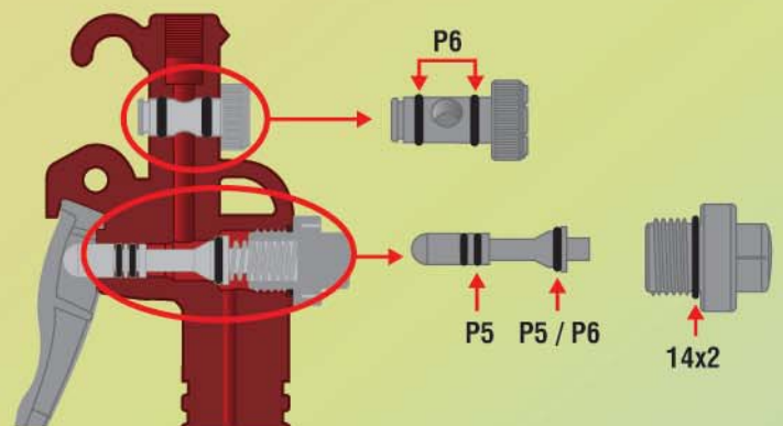
Sectional View
