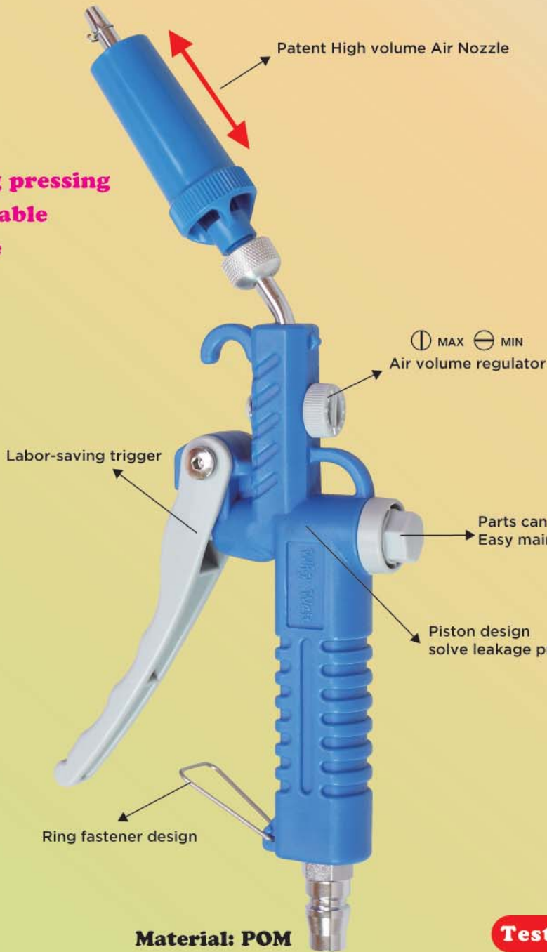
Traditional type air blow gun (with air volume regulator)
