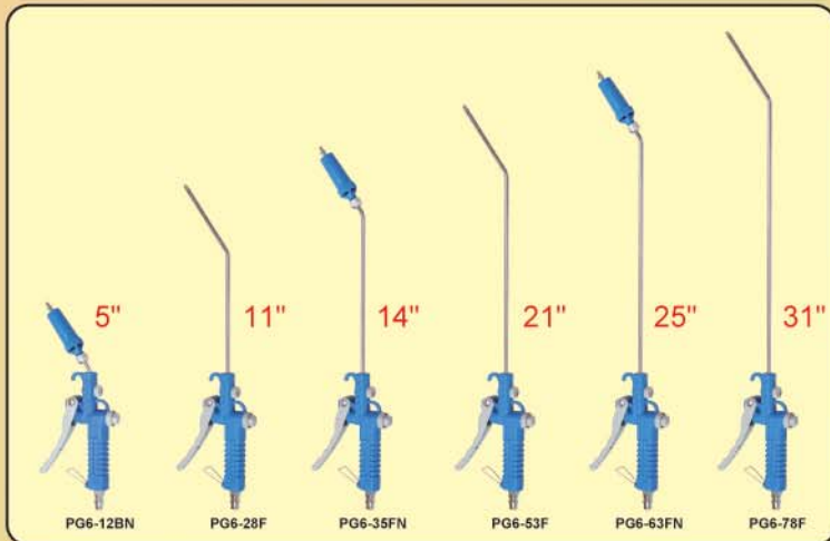
Traditional air blow gun attach turbo air nozzle
