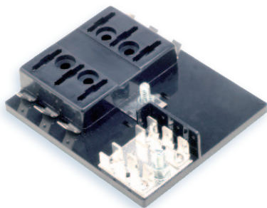
202-06U 6 Way Fuse Holder Terminal
