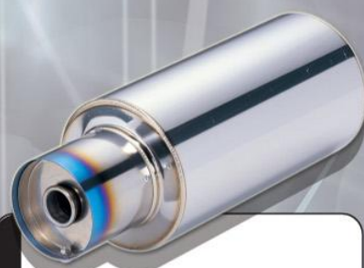
CR-7032T-BTT Ø63.5m/m(Ø2-1/2") Tip:TO-115R Flat
