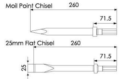
TH-2120/H(R) 4" Air Chipping Hammer
