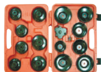
AMR978I 16PC CUP TYPE OIL FILTER WRENCH SET 65 - 108mm CUP RANGE, 3 LEG WRENCH (65 - 120mm)
