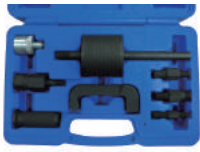
PUG490E 9PC INJECTION NOZZLE PULLER MERCEDES CDI ENGINES OM 611, 612, 613, ETC.
