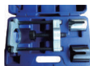
AMR1112E SUB - FRAME BUSH REMOVER & INSTALLER - MERCEDES BENZ
