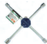
SSR788A 4 WAY LUG WRENCH (THIN WALL TYPE) SIZES: 17 x 19 x 21 x 23mm
