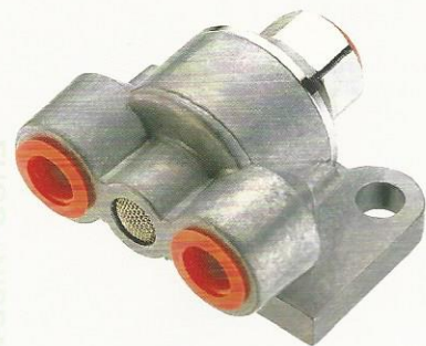
Quick Release Valve FUSO : 03342-56000 NISSAN : 45151-Z0001
