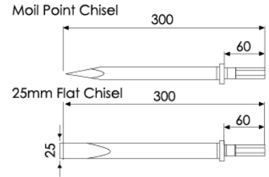
TH-2117/H(R) 4" Air Chipping Hammer
