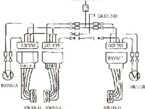
WIRING DIAGRAM: 3PCS SWITCHES
