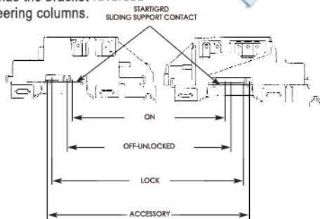
Fig. 1 AES-1111-35A Standard Steering Column
