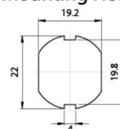
Mounting Hole
